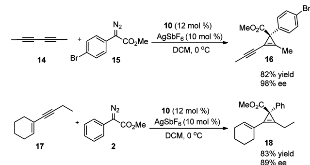
Scheme 1. Au(I)-Catalyzed Cyclopropanation of Electronically Activated Alkyl Alkynes
