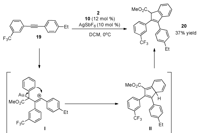
Scheme 3. Au(I)-Catalyzed Cyclopropanation of Electronically Activated Alkyl Alkynes
