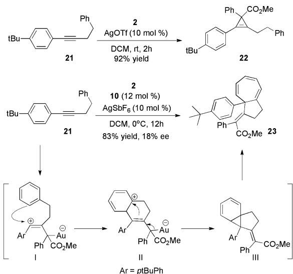
Scheme 3. Au(I)-Catalyzed Cyclopropanation of Electronically Activated Alkyl Alkynes
