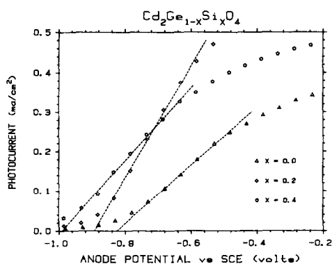
FIG. 2. Photoresponse under "white" xenon arc irradiation of 1.0 W/cm 2 in pH \approx 13 electrolyte.
