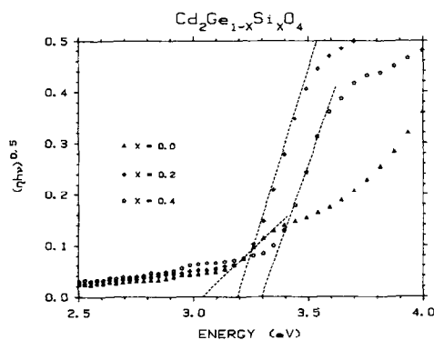
FIG. 3. Band gap determination based on the quantum efficiency measured at an anode potential of -0.2 V vs SCE in pH \approx 13 electrolyte.
