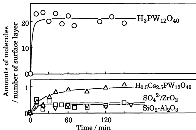
Fig. 2. Amounts of molecules held by the catalysts during the rearrangement of pinacol at 323 K.
