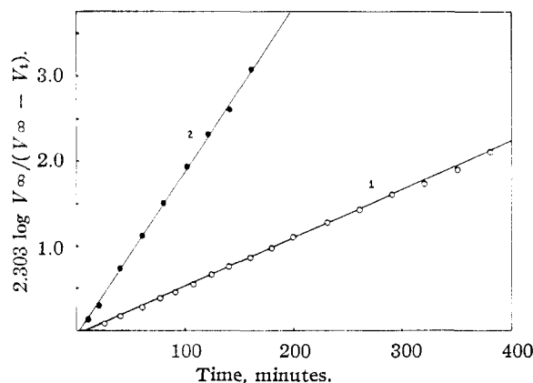
Fig. 1.—Decomposition of 0.01 M azo-bis-diphenylmethane in toluene: curve 1, 54°; curve 2, 64°.
