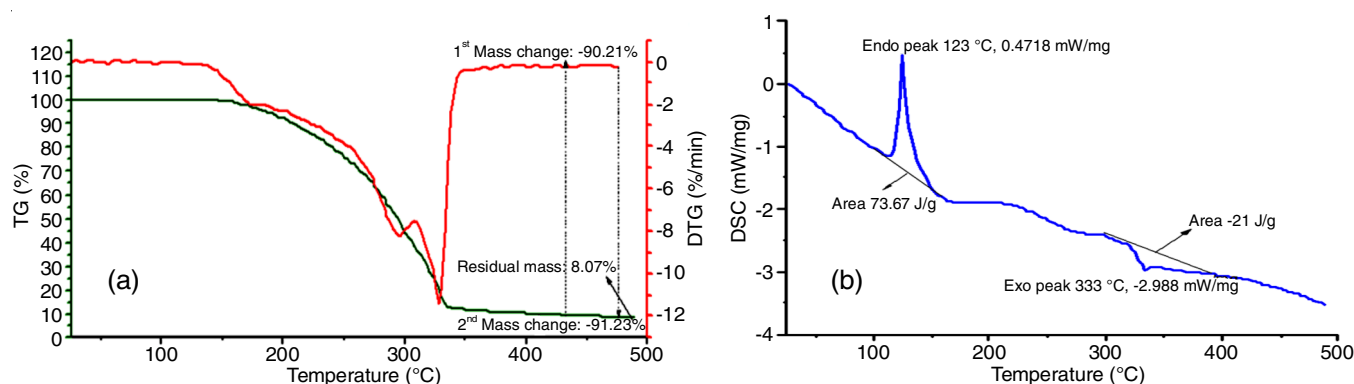
Fig. 2. (a) TG -DTA curve and (b) DSC curve of 4B2PMP
