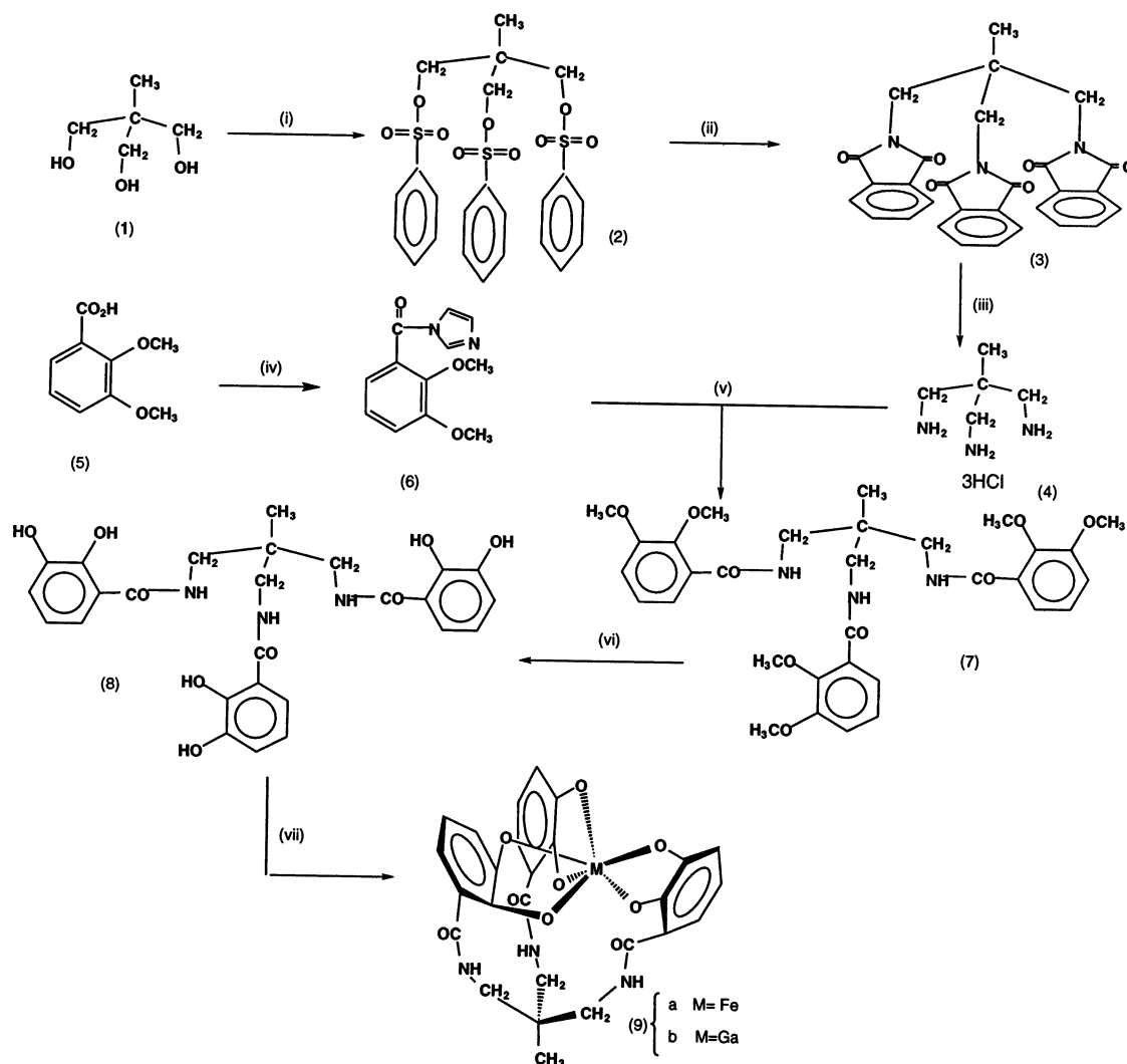
Scheme 1. Reagents and conditions: (i) PhSO_2Cl , pyridine; (ii) Potassium phthalimide, DMF; (iii) Autoclave, 170^\circ C , KOH; (iv) CDI, CH_2Cl_2 ; (v) Et_3N , CH_2Cl_2 ; (vi) BBr_3 , CH_2Cl_2 ; (vii) Fe(acac)_3 , CH_2Cl_2 , or Ga(NO_3)_3 , CH_2Cl_2 .
