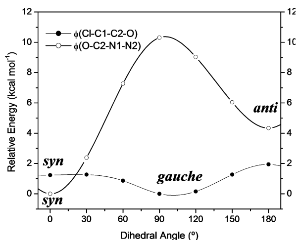
Figure 1. Calculated potential energy curves for the internal rotation around the \text{C}1-\text{C}2 and \text{C}2-\text{N}1 bonds of \text{ClF}_2\text{CC}(\text{O})\text{N}_3 by using the B3LYP/6-311+G(d) method. The relax scan of the potential energy surface was performed by rotating the dihedral angle, either \text{C}1-\text{C}2-\text{O} or \text{O}-\text{C}2-\text{N}1-\text{N}2 , in steps of 30^\circ while optimizing the rest of the molecule.
