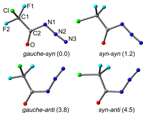
Figure 2. Optimized structures with atomic labeling and relative energies ( \text{kcal mol}^{-1} ) for the minimum energy conformations of \text{ClF}_2\text{CC}(\text{O})\text{N}_3 at the B3LYP/6-311+G(3df) level of theory.
