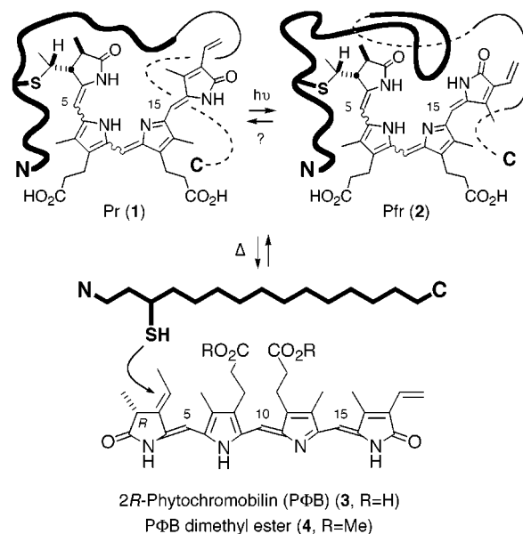
Figure 1. Interconversion of Pr ( 1 ), Pfr ( 2 ), and PΦB ( 3 ).
