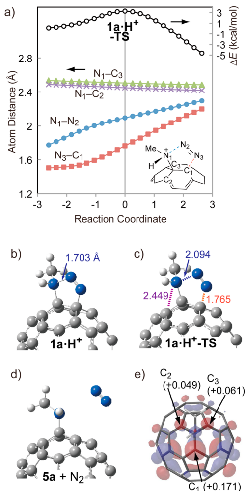
Figure 4. (a) Energies and atomic distances of IRC calculation (B3LYP/6-31G(d) with solvent parameters) for the acid-catalytic denitrogenation. The energies are relative to the initial state 1a·H + . (b) Geometry of N 1 -acidified 1a·H + . (c) Transition state geometry ( 1a·H + -TS ) of denitrogenation of 1a·H + . (d) Geometry of aminofullerenyl cation 5a (and N 2 ) derived from the optimization of the IRC forward-edge structure ( s = 2.64). (e) LUMO orbital distribution and natural bonding orbital charge (in parentheses) of the ionic intermediate 5a .
