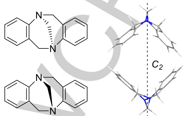
Figure 1. Chemical and simulated three-dimensional structure (Chem3D 15.0, MM2) of TB's framework (top: R,R; bottom: S,S)
