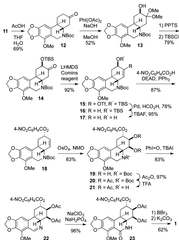
Scheme 3. Total Synthesis of (+)- trans -Dihydronarciclasine ( 1 )
