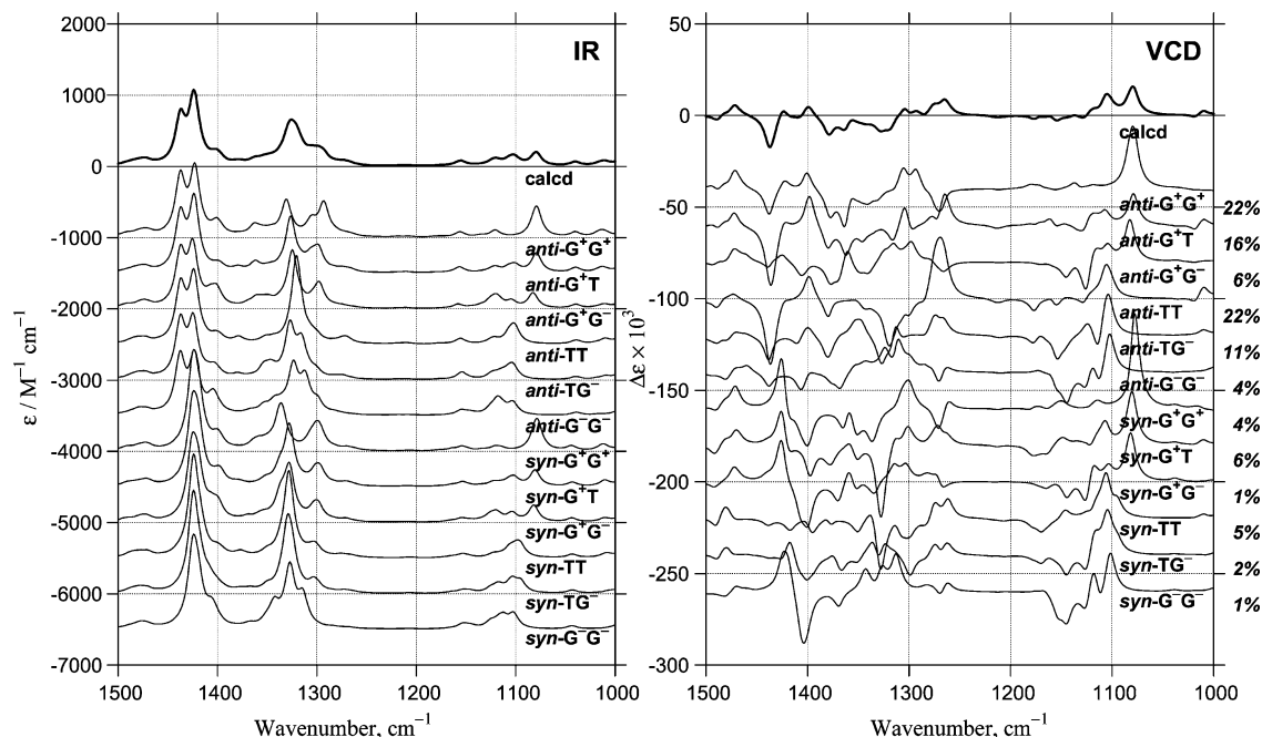
Figure 6. Calculated IR (left) and VCD (right) spectra of 2b^{\bullet+} . The DFT-calculated IR and VCD profiles of each conformer and the relative contribution estimated from the Gibbs free energies are shown. Y-axis of the calculated spectra is shifted for clarity.
