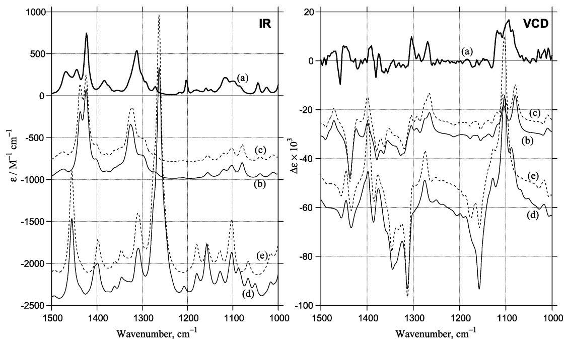
Figure 5. Experimental and calculated IR (left) and VCD (right) spectra of 2b^{\bullet+} . (a) Observed; (b) DFT simulation using all 12 conformers; (c) DFT simulation using 4 selected conformers; (d) HF simulation using all conformers; (e) HF simulation using 4 conformers. Y-axis of the calculated spectra is shifted for clarity.
