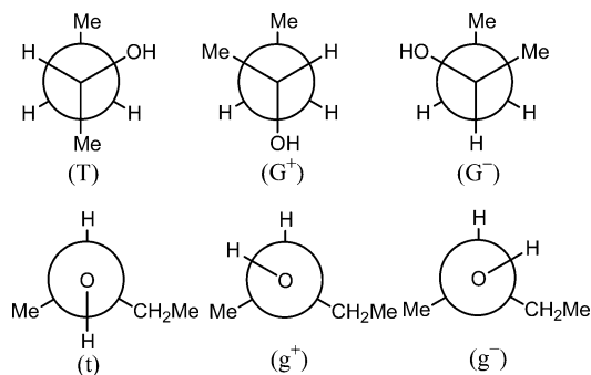
CHART 4: Conformers of ( R )-2-Butanol with Different Dihedral Angles around the C–C–C*–C and H–C*–O–H Bond
