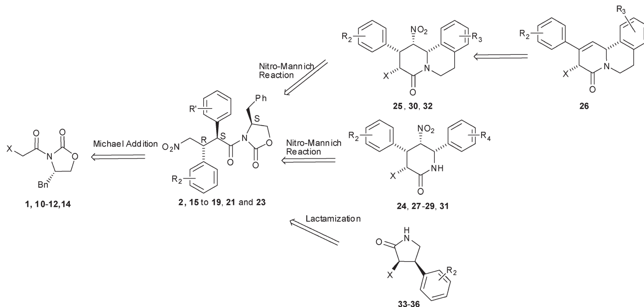
Scheme 1 Diversity oriented synthesis of N-heterocycles.
