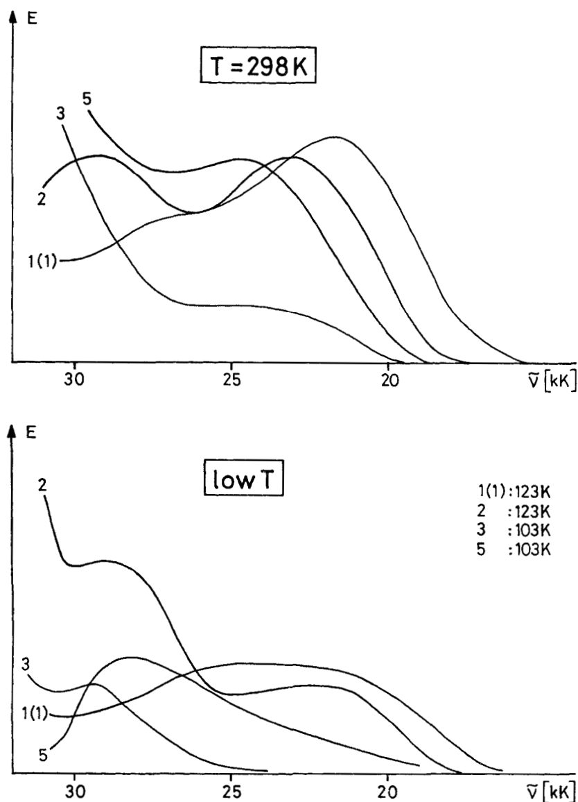
Fig. 3. CT-spectra in fluid and glassy ( n -BuCl/CH 2 Cl 2 , 3:2 by vol.) medium. (Arbitrary concentrations of D, [TCNE] = 6.43 \times 10^{-3} M)
