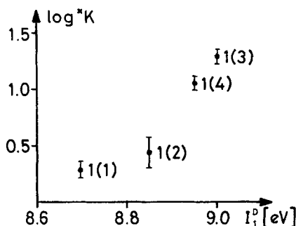
Fig. 5. Correlation of complex stability ( *K_{ap} ) and donor capacity ( I_1^D )
