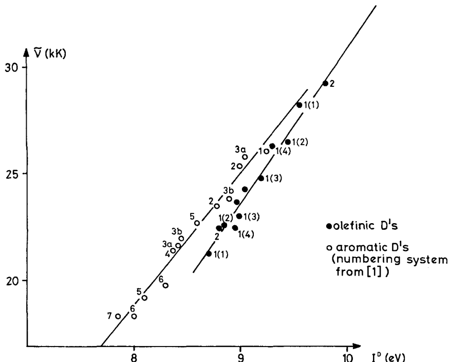
Fig. 4. Plot of h\nu^{CT} vs. I^D for olefinic and aromatic donors ( A = \text{TCNE} )
