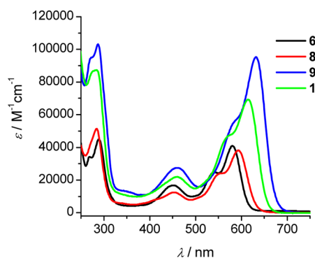
Figure 3. UV/vis absorption spectra of perylene derived compounds measured in CH 2 Cl 2 at 298 K at concentrations in the range of 10 -5 M.
