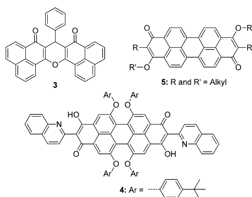
Figure 2. Structures of literature known phenalenone derivative 3 and benzoperylenes 4 and 5 .
