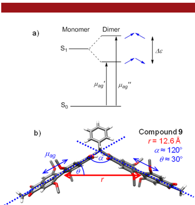
Figure 4. (a) Splitting of energy levels in an oblique excitonic coupling showing the excitonic coupling \Delta\epsilon and transition strengths \mu_{ag}' and \mu_{ag}'' . (b) MMFF94 energy minimized structure of covalently linked perylene dimer 9 , and parameters \alpha , \theta , r , and \mu_{ag} ( t Bu-phenyl groups omitted for clarity).
