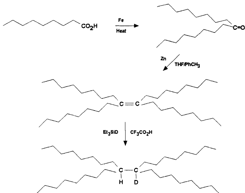
Scheme 2: Synthesis of 9- d -9,10-dioctyloctadecane
