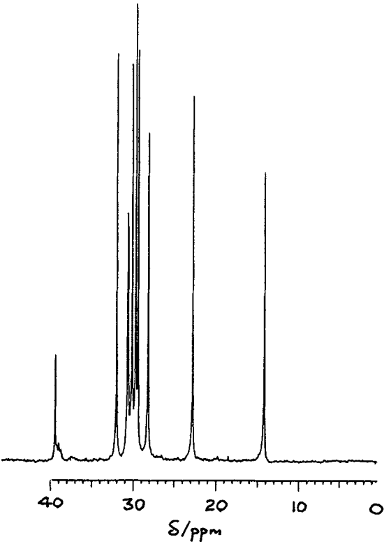
Figure 3: 13 C-NMR Spectrum of 9,10-dioctyloctadecane
