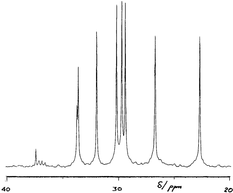
Figure 4: Detail of 13 C-NMR Spectrum of 9-d-9,10-dioctyloctadecane (20-40 ppm region)
