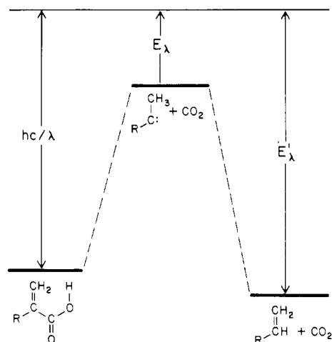
Figure 2. Schematic energy level diagram for the fragmentation of acrylic acid ( R = H ) and methacrylic acid ( R = CH_3 ). See text for explanation of notation.
