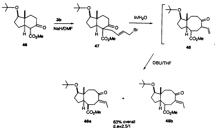
Scheme 7.
