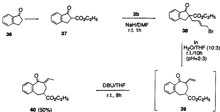
Scheme 5.
