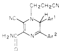
13a, Ar 1 = Me 3 CH; Ar 2 = 4-NO 2 C 6 H 4 b, Ar 1 = 4-Me 2 CHC 6 H 4 ; Ar 2 = 4-CNC 6 H 4
