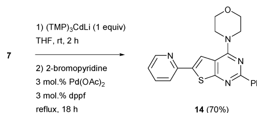
Scheme 2 Deproto-cadmiation (using (TMP) 3 CdLi) followed by cross-coupling.
