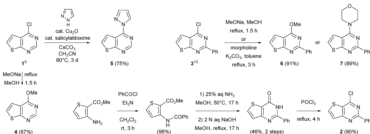
Scheme 1 Synthesis of the substrates 1–7.
