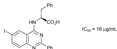
Scheme 3 Cytotoxic activity of 2-(6-iodo-2-phenylquinazolin-4-ylamino)-3-phenylpropanoic acid.
