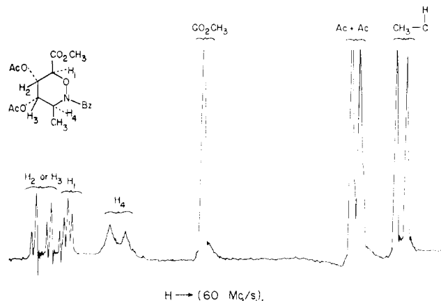
Fig. 2.—Spectrum of the diacetate of XVI in chloroform; tentative assignment.
