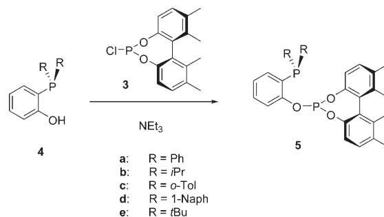
Scheme 1. Synthesis of phosphane-phosphites 5 .
