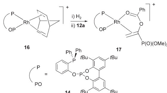
Scheme 4. Synthesis of 17 .
