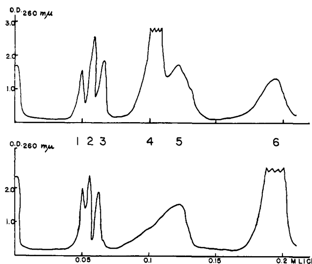
Figure 2. Comparative elution patterns in DEAE Cl - chromatography of condensation products in the synthesis of coenzyme A (top) and selenocoenzyme A (bottom). Peak 4: coenzyme A-SH, note the absence of a corresponding selenocoenzyme A-SeH peak; peak 6: coenzyme A disulfide and selenocoenzyme A diselenide. For details see text.
