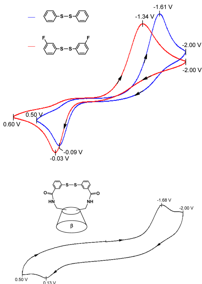
Figure 3. Cyclic voltammograms (100 mV/s) in Me 2 SO of diphenyl disulfide (blue, upper), bis(3-fluorophenyl) disulfide (red, upper), and \beta -cyclodextrin disulfide (lower). Peak potentials are indicated.
