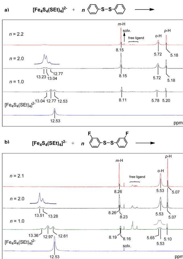
Figure 4. 1 H NMR spectra (600 MHz) in the downfield region for the reaction between 14 mM [Fe 4 S 4 (SET) 4 ] 2- and n equiv of (a) diphenyl disulfide and (b) bis(3-fluorophenyl) disulfide in (CD 3 ) 2 SO at ~25 °C. The signal assignments of bound arylthiolate ligands are indicated; solv = DMF.
