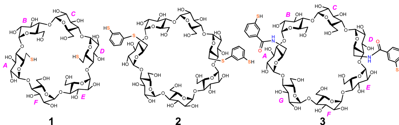
Figure 1. Schematic structures of cyclodextrin dithiols: 6 A ,6 D -(CH 2 SH) 2 -6 A ,6 D -dideoxy- \alpha -cyclodextrin (1), 6 A ,6 D -(3-SC 6 H 4 -1-SH) 2 -6 A ,6 D -dideoxy- \beta -cyclodextrin (2), 6 A ,6 D -(3-NHC(O)C 6 H 4 -1-SH) 2 -6 A ,6 D -dideoxy- \beta -cyclodextrin (3). Abbreviations of doubly deprotonated forms: \alpha -CD-(CH 2 S) 2 , \beta -CD-(1,3-SC 6 H 4 S) 2 , \beta -CD-(3-NHC(O)C 6 H 4 -1-S) 2 . CD = cyclodextrin.
