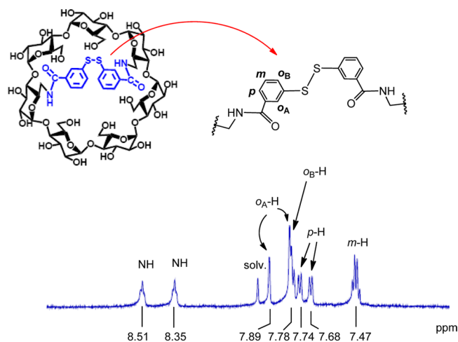
Figure 2. Schematic structure of \beta -cyclodextrin disulfide and designation of the aromatic protons and the 1 H NMR spectrum (600 MHz) of the downfield region in (CD 3 ) 2 SO. Signal assignments are indicated; solv = DMF.
