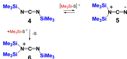
Scheme 2. Isomerization of Bis-silylated Carbodiimide Catalyzed by [\text{Me}_3\text{Si-S}]^+ (S = Solvent)
