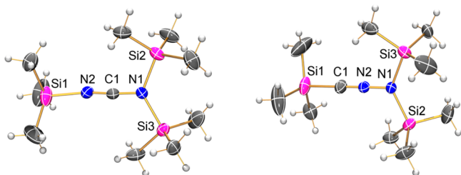
Figure 2. ORTEP drawing of the molecular structure of the [(Me 3 Si) 2 NCN(SiMe 3 )] + ion in 6[B(C 6 F 5 ) 4 ] − (left) and the [(Me 3 Si) 2 NNC(SiMe 3 )] + ion in 9[B(C 6 F 5 ) 4 ] − (right) in the crystal. Thermal ellipsoids with 50% probability at 173 K. Selected bond lengths (Å) and angles (°): for 6, C1–N2 1.18(1), N1–C1 1.279(2), N1–Si2 1.835(1), N1–Si3 1.838(1), C1–N2–Si1 159.4(9), C1–N1–Si2 115.01(8), C1–N1–Si3 116.04(8), Si2–N1–Si3 128.93(6), N1–C1–N2 173.3(5); for 9, N1–N2 1.309(2), N2–C1 1.143(2), Si2–N1 1.818(1), Si3–N1 1.816(1), Si1–C1 1.897(2), C1–N2–N1 179.3(1), N2–N1–Si3 113.76(8), N2–N1–Si2 114.89(8), N2–C1–Si1 174.6(1), Si3–N1–Si2 131.34(6).
