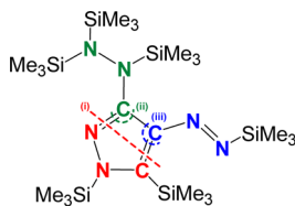
Scheme 8. Retrosynthetic Analysis of 7: (i) C–C Coupling Prior to [3+2] Cycloaddition, (ii) C–C Coupling Prior to [4+1] Cycloaddition, and (iii) C–N Coupling Prior to [4+1] Cycloaddition
