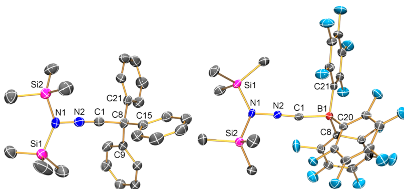
Figure 4. ORTEP drawing of the molecular structures of 10 (left) and 11 (right) in the crystal. Thermal ellipsoids with 50% probability at 173 K. Selected bond lengths (Å) and angles (°): for 10 , N2–C1 1.145(4), N2–N1 1.334(4), C1–C8 1.480(4), N1–Si2 1.818(3), N1–Si1 1.823(3), C1–N2–N1 179.1(3), N2–N1–Si2 111.9(2), N2–N1–Si1 113.3(2), Si2–N1–Si1 132.6(2); for 11 , N2–C1 1.145(2), N2–N1 1.331(2), N1–Si1 1.805(1), N1–Si2 1.805(1), C1–B1 1.617(2), C1–N2–N1 177.7(1), N2–N1–Si1 114.91(6), N2–N1–Si2 111.52(6), Si1–N1–Si2 133.35(4).
