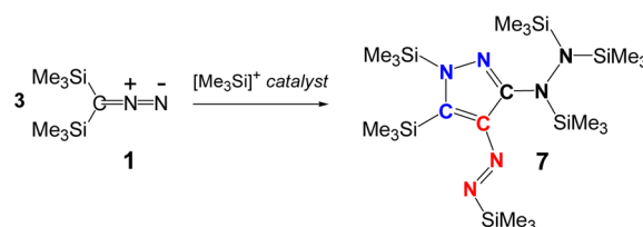
Scheme 3. Catalytic Trimerization of Bis-silylated Diazomethane 32
