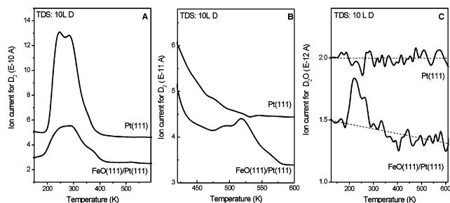
Figure 2. (A) D_2 TDS spectra, (B) zoom-in D_2 TDS spectra between 420 and 600 K, and (C) D_2O TDS spectra of Pt(111) and FeO(111)/Pt(111) inverse model catalyst exposed to 10 L of D at 120 K. The dashed lines indicate the baselines.
