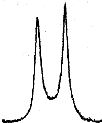
Fig. 1. ^{19}\text{F} NMR spectrum of perfluoroisopropylsilver in acetonitrile ( \text{CF}_3 group).
