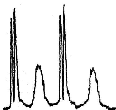
Fig. 3. ^{19}\text{F} NMR spectrum of perfluoro-tert-butylsilver in 1,2-dimethoxyethane.
