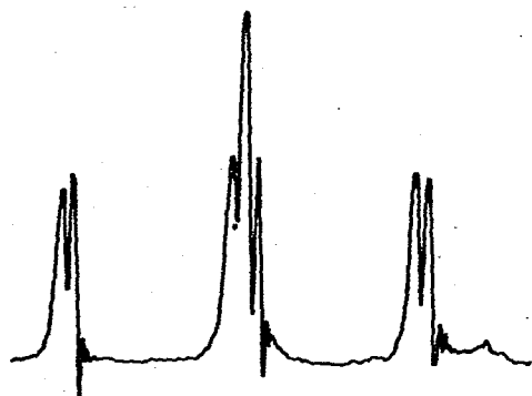
Fig. 1. ^{19}\text{F} NMR spectrum of perfluoroisopropylsilver in acetonitrile ( \text{CF}_3 group).
