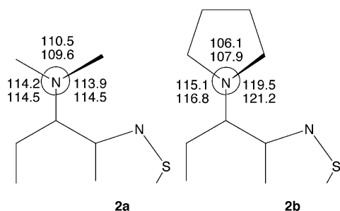
Figure 2. Angular geometry around amino nitrogens of 2a (a) and 2b (b). Estimated standard deviations for bond angles are 0.1–0.3° for 2a and 0.4–0.7° for 2b .
