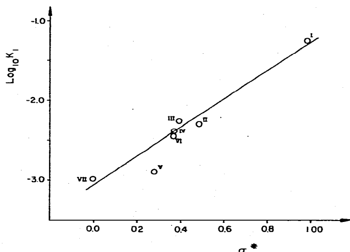
Fig. 1. \sigma^* \rho^* correlation for the monometallation of alkylphenylacetylenes (I–VII).
