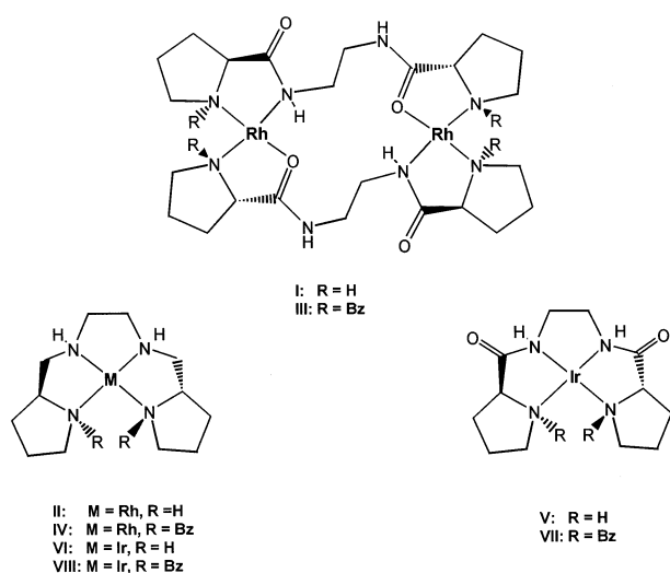
Fig. 2. Proposed structures for the rhodium and iridium complexes I–VIII .
