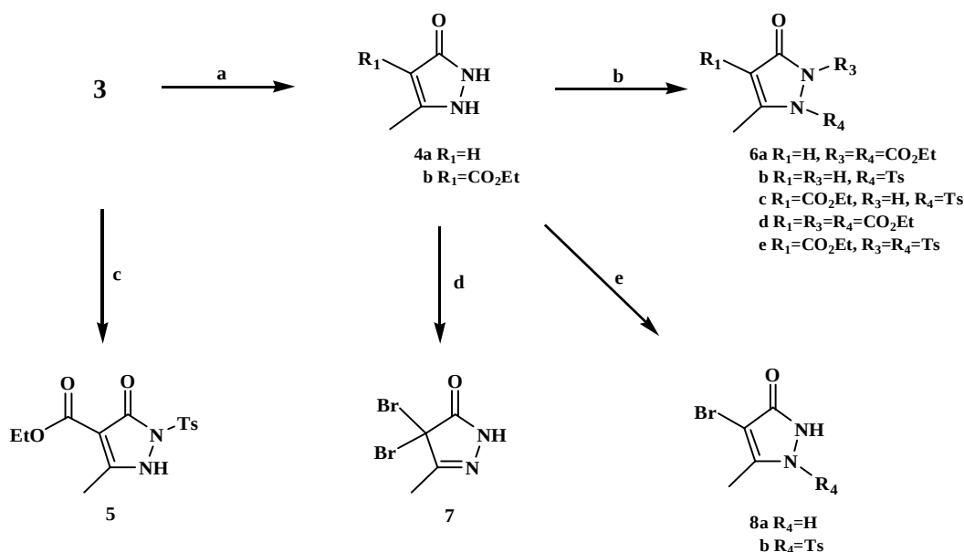
Scheme 1. Reagents and conditions: (a) Method A: \text{H}_2\text{NNH}_2 (80%)/EtOH; Method B: \text{H}_2\text{NNH}_2 (pH=7), EtOH/ \text{H}_2\text{O} ; Method C: \text{H}_2\text{NNH}_2 (55%)/HOAc; Method D: \text{H}_2\text{NNH}_2\cdot\text{HCl} /EtOH; (b) Method A: \text{ClCO}_2\text{Et} , TEA/ \text{CH}_2\text{Cl}_2 ; Method B: TsCl, TEA/ \text{CHCl}_3 ; (c) \text{H}_2\text{NNH-Ts} /HOAc; (d) NBS, pyridine/ \text{CH}_2\text{Cl}_2 ; (e) NBS, NaH (60%)/THF.
