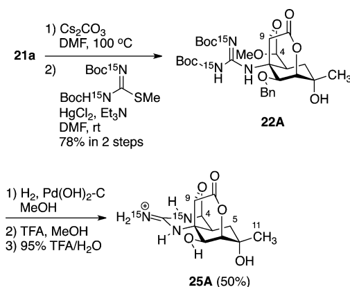
Scheme 7. Synthesis of ^{15}\text{N}_2 -labeled 4,9-Anhydro-5,11-dideoxytetradotoxin (25A)
