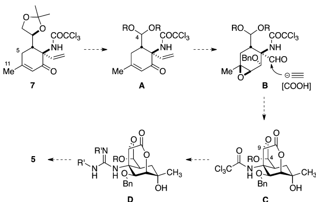
Scheme 1. Improved Synthetic Plan for (–)-5,11-Dideoxytetrodotoxin (5)
