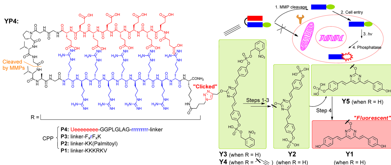
Figure 2. Overall strategy of the four CPP-conjugated 2P fluorogenic substrates, YP1 to YP4 . They were used for subcellular bioimaging of endogenous phosphatase activities in mammalian cells and Drosophila brains. The 2P reporter in all four conjugates was in the “caged” form (similar to Y3 , where R = H). Sequences of the four CPPs ( P1 to P4 ) were shown by their single-letter amino acid alphabets. Unnatural AAs were represented as F x = L-cyclohexylalanine; r = D-Arg; e = D-Glu; U = succinic acid. The full structure of YP4 is shown, with the negatively charged D-Glu/succinic acid and the positively charged D-Arg highlighted in red and blue, respectively. MMP cleavage site in YP4 is indicated. In the tumor cell-specific approach, membrane-bound MMPs first cleaved the masking “red” peptide fragment (Step 1), exposing the “blue” CPP and delivering the probe into the cells (Step 2). Subsequent UV irradiation (Step 3) released the phosphatase-responsive probe Y2 , which was dephosphorylated by endogenous PPs, generating highly fluorescent and localized Y1 (Step 4), possibly through the monophosphorylated intermediate Y5 .
