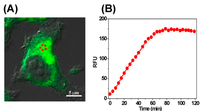
Figure 5. (A) One-photon excited fluorescence microscopy of live HepG2 cells treated with Y3 (10 \mu\text{M} ). Following 2-min UV irradiation, the cells were imaged over the course of 120 min with 60-s intervals ( \lambda_{\text{ex}} = 405 \text{ nm} ; PMT range: 460–550 nm). The image shown was taken at the 80-min time point. Scale bar = 5 \mu\text{m} . (B) Graphical representation of time-dependent changes in fluorescence intensity at the circled position in panel A.
