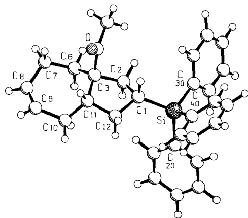
Figure 3. Molecular structure of 11c in the crystal (SCHAKAL representation; arbitrary numbering). Selected bond lengths [Å]: C1–C2 1.543(5), C2–C3 1.543(5), C3–C11 1.557(5), C11–C12 1.546(4), C1–C12 1.534(6), Si–C1 1.879(4), Si–C20 1.878(3), Si–C30 1.884(4), Si–C40 1.876(3).
