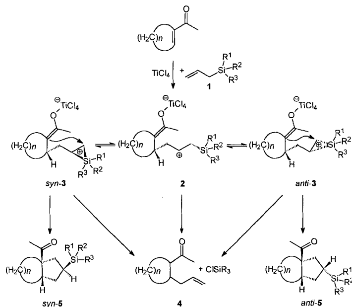
Scheme 1. Proposed mechanism of the [3+2] cycloaddition.
