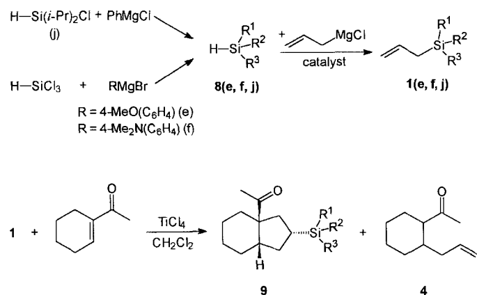
Scheme 3. Synthesis of allylsilanes 1 and [3+2] cycloadditions to silylbicyclo[4.3.0]nonanes 9 .
