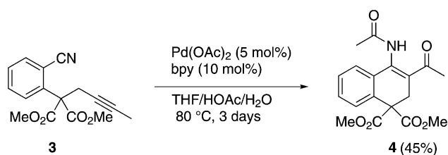
Scheme 1. Cyclization of dimethyl 2-(but-2'-ynyl)-2-(o-cyanophenyl)malonate. Reaction conditions: 3 (0.3 mmol), Pd(OAc) 2 (5 mol%) and bpy (10 mol%) were dissolved in THF (2 mL), HOAc (0.5 mL) and H 2 O (0.1 mL), then the mixture was stirred at 80 °C for 3 days.
