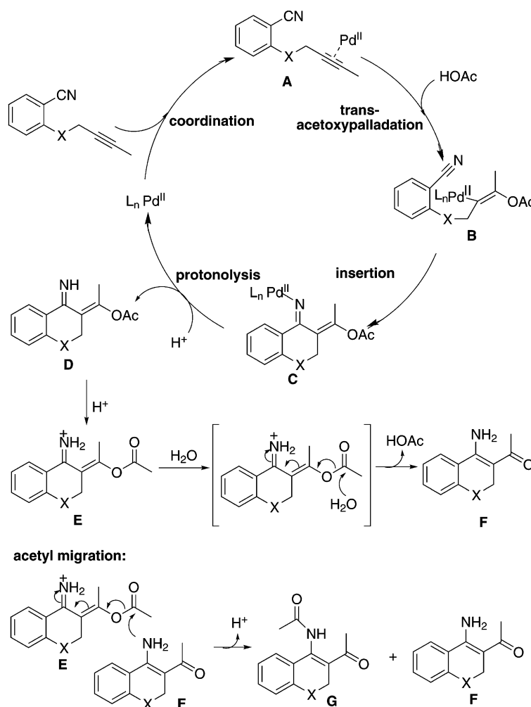
Scheme 2. A plausible mechanism for the palladium(II)-catalyzed tandem cyclization reaction.
