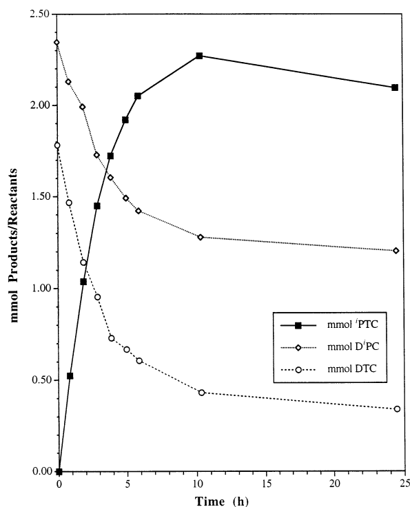
Fig. 1. Reaction profile of the metathesis of D'PC and DTC catalyzed by V(O)(O^iBu)_3 , 3 .
