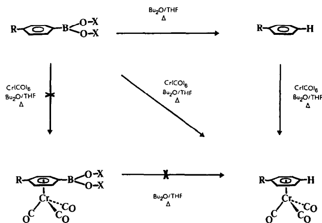
Fig. 1. Proposed reaction scheme for protodeboronation reactions in \text{Bu}_2\text{O}/\text{THF} . (X = H for arylboronic acids and X = remainder of the heterocyclic \text{B}_3\text{O}_3 system in arylboroxines; R = H, Me, Br).
