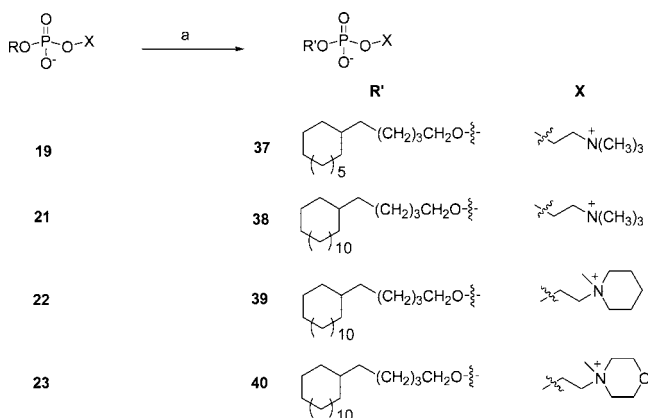
Scheme 7 a
