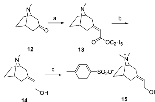
Scheme 3 a
