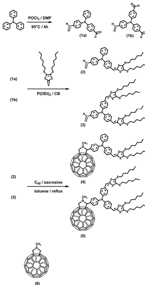
Scheme 1 Synthesis of 4 and 5 as well as reference 6 .
