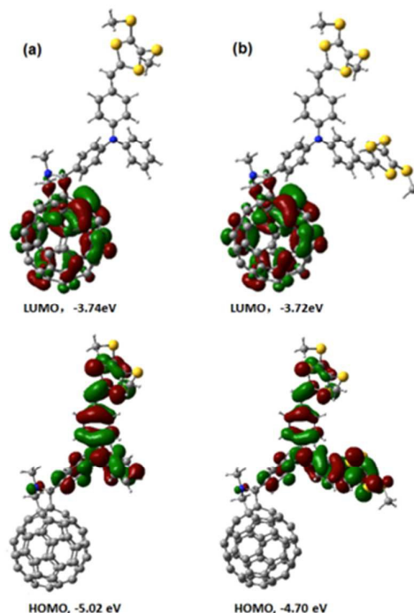
Figure 3. Optimized structures and electron densities of LUMOs and HOMOs of (a) 4 and (b) 5 calculated at B3LYP/3-21G level of theory.
