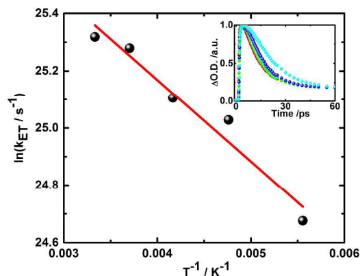
Figure 6. Plot of rate constant for the charge recombination of the singlet radical ion pair state vs T^{-1} for 5 in 2-methyl THF upon photoexcitation at 387 nm. Linear fit is shown in red. Inset: Corresponding time-absorption profiles at 600 nm obtained at 300 K (black), 270 K (red), 240 K (green), 210 K (blue), and 180 K (cyan).
