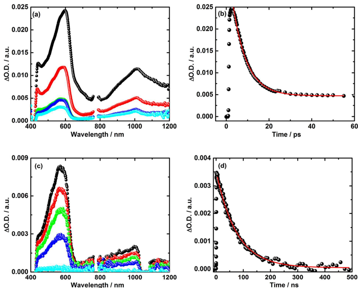
Figure 4. (a) Transient absorption spectra of 5 in argon saturated THF upon fs-laser photolysis (387 nm, 400 nJ / pulse) with time delays of 2 ps (black), 10 ps (red), 100 ps (green), 1000 ps (blue), and 5000 ps (cyan) after the laser pulse. (b) Corresponding time absorption profile (black) and exponential decay fit (red) at 590 nm. (c) Nanosecond transient absorption spectra of 5 in argon saturated THF upon laser photolysis (387 nm, 400 nJ / pulse) with time delays of 5 ns (black), 25 ns (red), 50 ns (green), 100 ns (blue) and 500 ns (cyan) after the laser pulse. (d) Corresponding time absorption profile (black) and exponential decay fit (red) at 590 nm.
