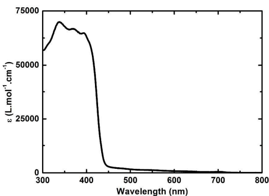
Figure 2. Absorption spectrum of 5 in toluene.
