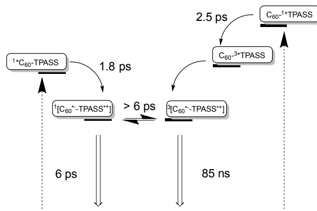
Figure 8. Simplified energy diagrams for 5 in THF illustrating on the left and on the right the different deactivation pathways upon photoexcitation of TPA-bis-dithiafulvene (TPASS) at 387, 420, and 568 nm and C_{60} at 387 and 420 nm, respectively. The energy of the radical ion pair state energy was determined as 1.25 eV for 5 from the one electron reduction of C_{60} as -1.19 V versus Fc/Fc^+ and the one electron oxidation of TPASS as +0.05 V versus Fc/Fc^+ and as 1.25 eV for 4 from the one electron reduction of C_{60} as -1.14 V versus Fc/Fc^+ and the one electron oxidation of TPASS as +0.11 V versus Fc/Fc^+ .
