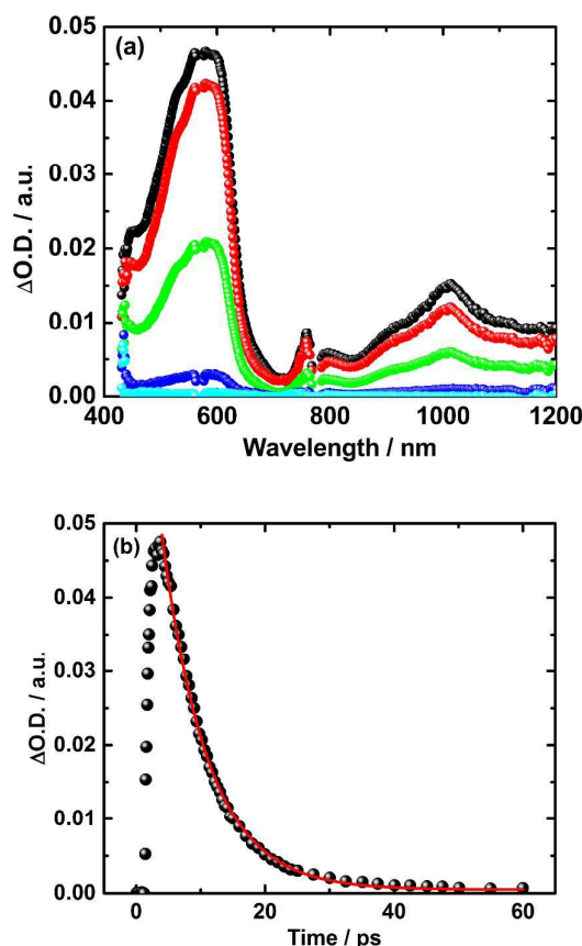
Figure 5. (a) Transient absorption spectra of 5 in argon saturated THF upon fs-laser photolysis (568 nm, 400 nJ / pulse) with time delays 2 ps (black), 5 ps (red), 10 ps (green), 25 ps (blue), and 100 ps (cyan) after the laser pulse. (b) Corresponding time absorption profile (black) and exponential decay fit (red) at 590 nm.
