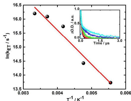
Figure 7. Plot of the rate constant for the charge recombination of the triplet radical ion pair state vs T^{-1} for 5 in 2-methyl THF upon photoexcitation at 387 nm. Linear fit is shown as in red. Inset: Corresponding time-absorption profiles at 600 nm obtained at 300 K (black), 270 K (red), 240 K (green), 210 K (blue) and 180 K (cyan).
