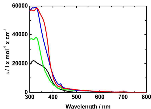
Figure 1. Absorption spectra of 2 (black), 6 (green), and 4 (red) in toluene. The blue line depicts the sum of the absorption spectra of 2 and 6 .
