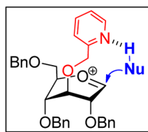
Chart 3. A Survey of Effects That Reduce Stereoselectivity by Disrupting the H-Bonding
