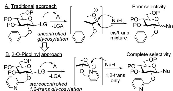
Scheme 1. Traditional Glycoside Synthesis Using Conventional 2- O -Benzyl Protection versus 2- O -Picolinyl-Assisted 1,2- trans -Glycosylation
