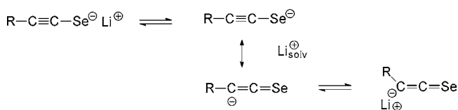
SCHEME 3 Equilibria of lithium alkynylchalcogenolates.
