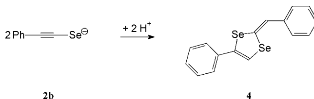
SCHEME 5 Synthesis of 4 .
