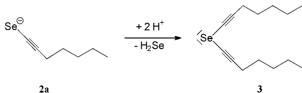
SCHEME 4 Formation of 3 .
