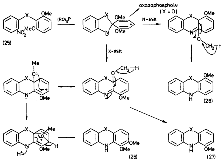
SCHEME 6 X = O or S
