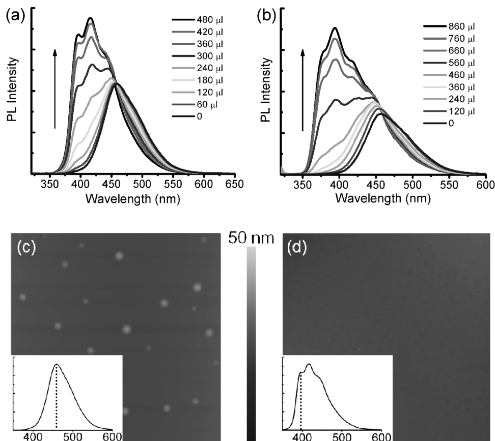
FIGURE 5 PL spectra of (a) Den 30-40 and (b) Den 50-40 in water with a consecutive adding of THF. The concentration of Den 30 , Den 50 , and Den 40 were 8.60 \times 10^{-6} , 8.60 \times 10^{-6} , and 5.26 \times 10^{-6} M, respectively. AFM images of mixed micelles, Den 30-40 , (c) before and (d) after addition of THF. The scanning areas of both are 10 \times 10 \mu\text{m} . Insets in Figure (c, d) represent the related PL emission spectra. The concentration of Den 30 and Den 40 for AFM images are 0.53 and 0.22 mM, respectively.
