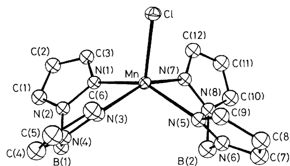
Figure. Structure of the anion [\text{MnCl}\{\text{H}_2\text{B}(\text{pz})_2\}_2]^-
