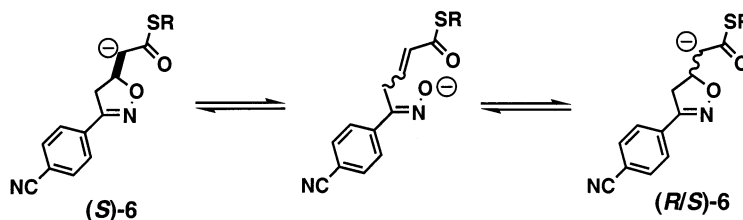
Scheme 2. Retro-Michael/Michael racemization mechanism of (S)-6 in the presence of base 4
