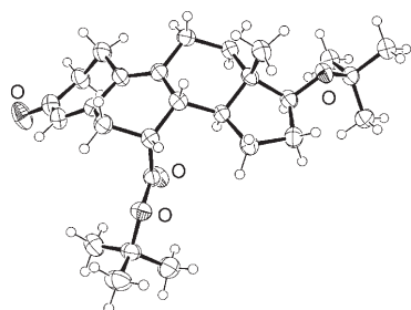
Figure 1. Structure of the steroid analogue trans - 27 in the crystal. [26]
