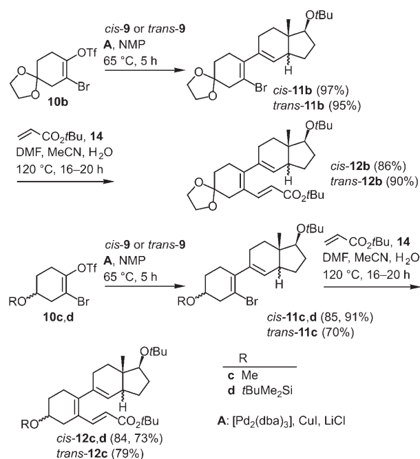
Scheme 5. Stille–Heck coupling sequences of substituted bromoenol triflates 10b–d with the bicyclononylstannanes cis - 9 as well as trans - 9 and tert -butyl acrylate to establish an array of tricyclic 1,3,5-hexatrienes as precursors for various steroid analogues.
