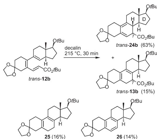
Scheme 7. Thermal 6\pi -electrocyclizations of the tricyclic 1,3,5-hexatriene trans - 12b and subsequent transformations of the initial product.
