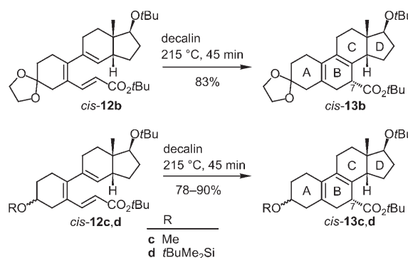
Scheme 6. Thermal 6 \pi -electrocyclization of tricyclic 1,3,5-hexatrienes cis - 12 with a subsequent [1,5]-hydrogen shifts to furnish differently 3-substituted steroidal systems with a diene B-ring. For further details see Table 3.
