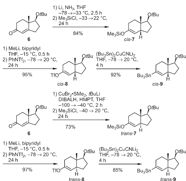
Scheme 2. Synthesis of the novel enantiomerically pure bicyclo[4.3.0]nonenylstannanes cis - 9 and trans - 9 starting from the bicyclic enone 6 .
