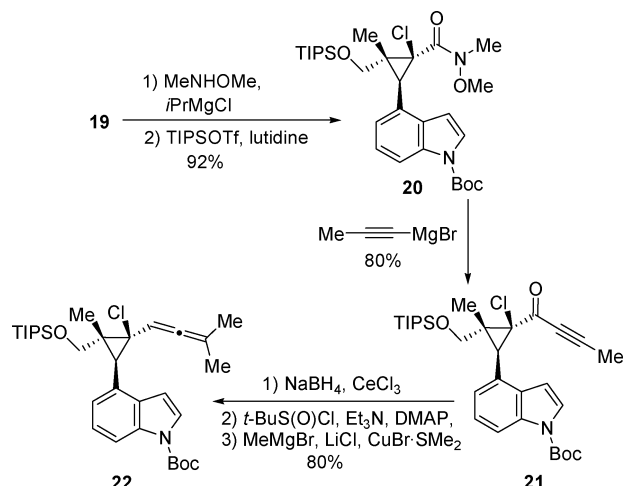
Scheme 4. Preparation of Pentasubstituted Allenylcyclopropane
