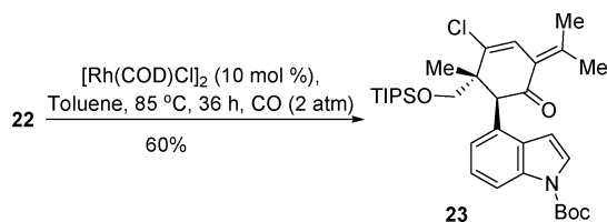
Scheme 5. Rh-Catalyzed [5 + 1] Cycloaddition of Allenylcyclopropane and CO
