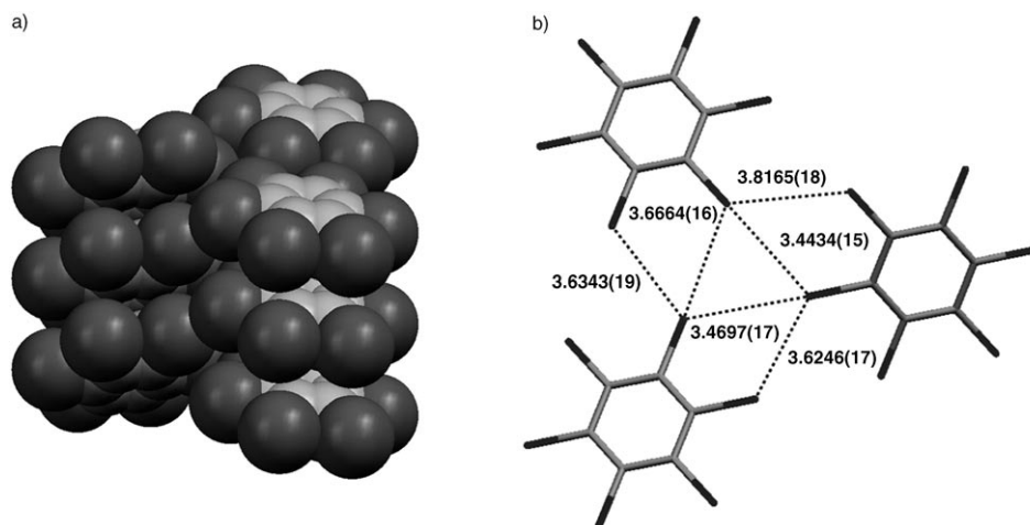
Figure 1. Monoclinic form for hexahalogenated benzenes: a) corrugated layer in C_6Cl_6 ; b) Cl \cdots Cl distances [Å] between stacks in C_6Cl_6 . Cl atoms are shown in dark grey and C atoms in light grey.
