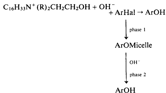
Scheme 1. R = Me, Et, Bu and Hal = Cl for compounds 1–4 or F for compounds 1a, 4a, 5 and 6
