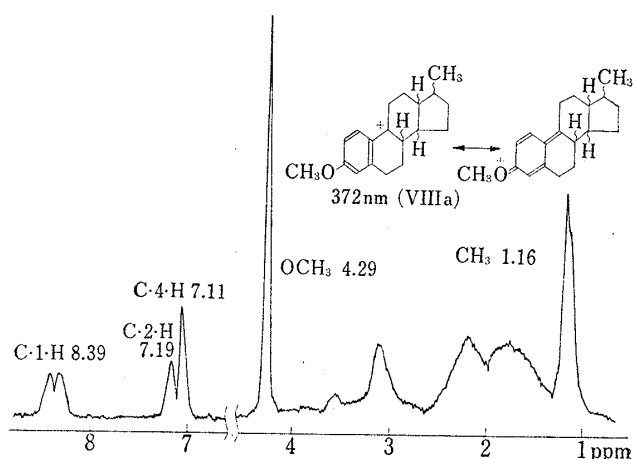
Fig. 5. NMR Spectrum of Carbonium Ions in Concentrated Sulphuric Acid
